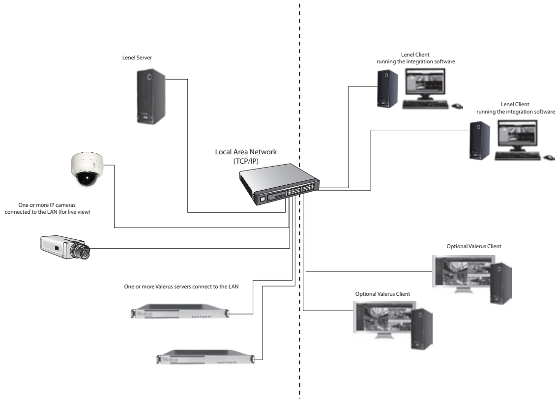
Typical Lenel OnGuardS2/Vicon Valerus Network Setup
